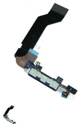
Flex with accessory connector + charge + data iPhone 4S black
